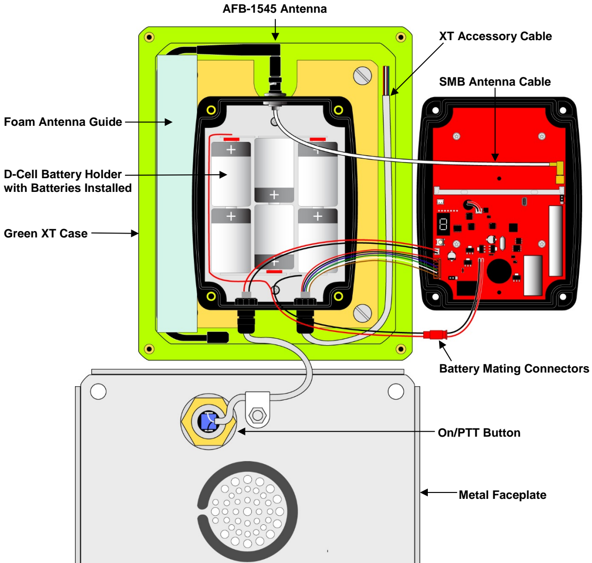
FIG-3: XT Callbox Assembly
